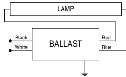
For 3-lamp, 2-lamp and 1-lamp application individually cap red and blue leads
