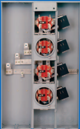
4 gang 200A per position All-In-One Meter
