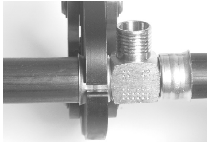
Figure 2 – Placing Jaw Squarely Onto PureFlow® Fitting
