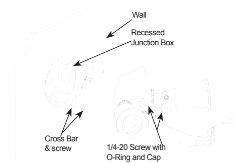
FIG 2 RECESSED JUNCTION BOX INSTALLATION
