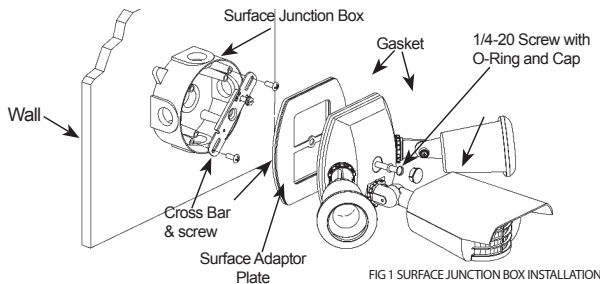
FIG 1 SURFACE JUNCTION BOX INSTALLATION
