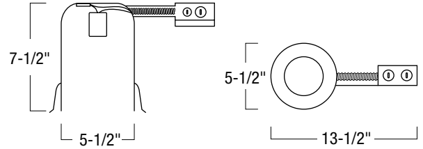
Ceiling Cut-out
