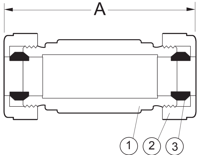
Pictured Brass Compression Coupling Cut-away
