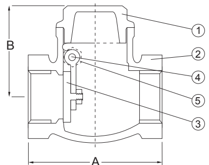
Pictured Model T-750 Cut-away
