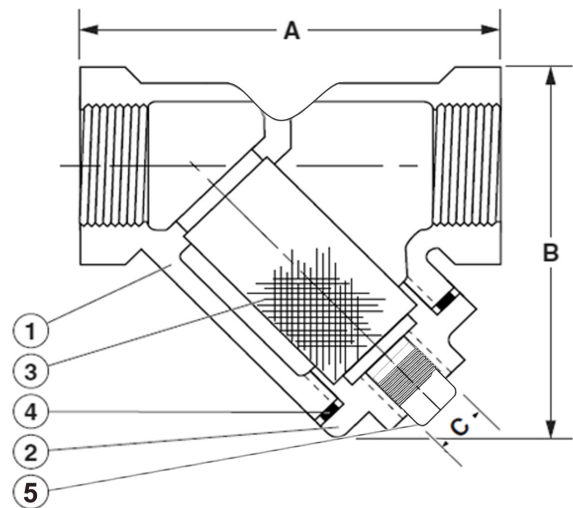
Pictured T-17 Cut-away
