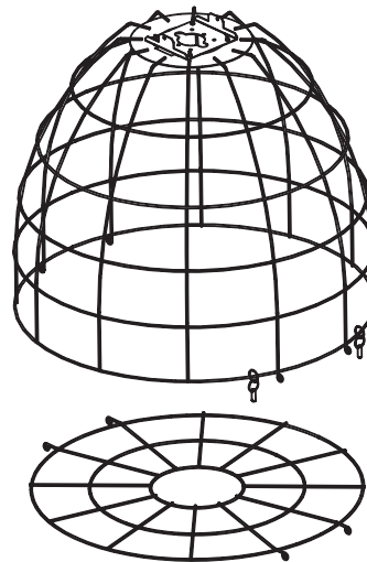
FIG. 20 FWG FULL WIRE GUARD FOR ACRYLIC REFLECTORS TRIBAY/SUPERBAY
