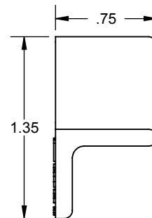
Model #212 (3/4" CTS)
