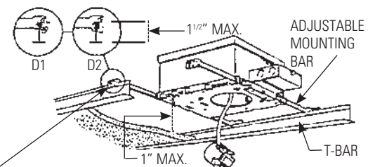
FIG.D Position notched areas of adjustable mounting bar on top of T-bar for proper spacing to finished ceiling. Lock mounting bars by bending tab underneath T-bar bead (FIG. D1), or use screw for round T-bar bead to lock bars, (FIG. D2)
