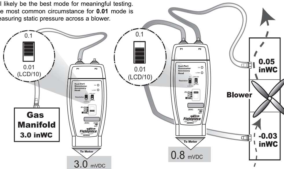
Static pressure across a blower (0.01 resolution mode) 0.8mVDC / 10 = 0.08inWC
