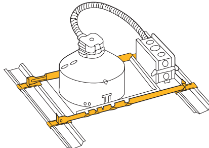
517 Series Light Fixture Suspension Bars
