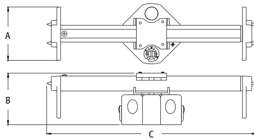
For Joist or Rafters 16" to 24" on center
