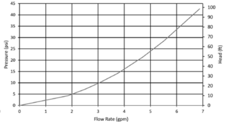
240HX3 PRESSURE LOSS
