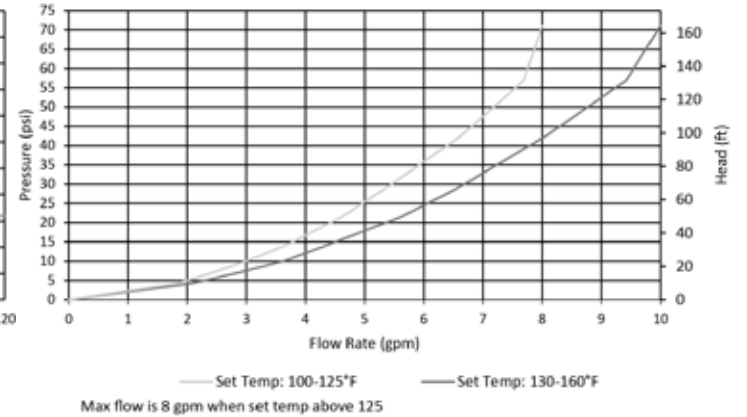
540HX3 PRESSURE LOSS
