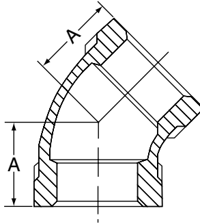
FIGURE 3102 - 45° ELBOW
